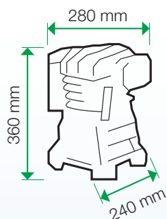
A49B pump
